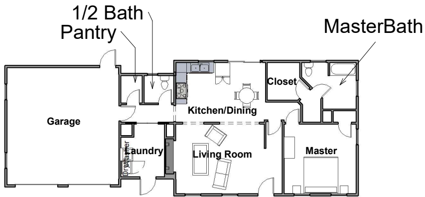
① Lvl1 Org. 3/32" = 1'-0"
